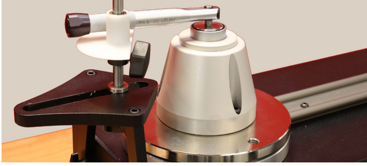
Flanş Tork Sensör (FMT) Flange Mounted Transducers
